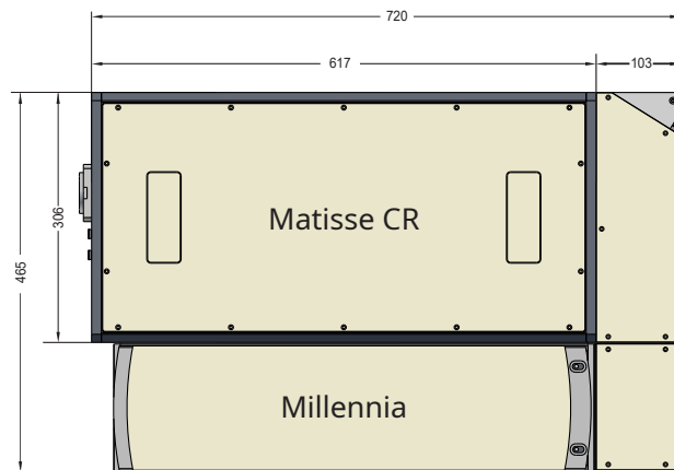
Matisse CR (Top view) (with Millennia eV 25W pump laser)
