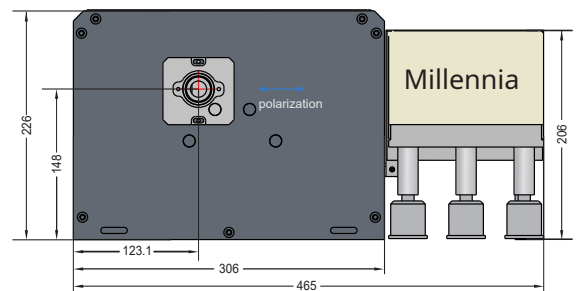
Matisse CR (Side view)
